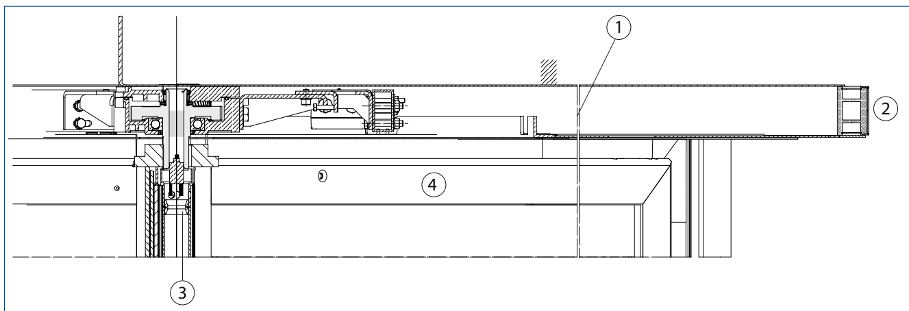
1 = Ceiling construction | 2 = Canopy profile | 3 = Swivelling axis | 4 = Side-hung leaf
