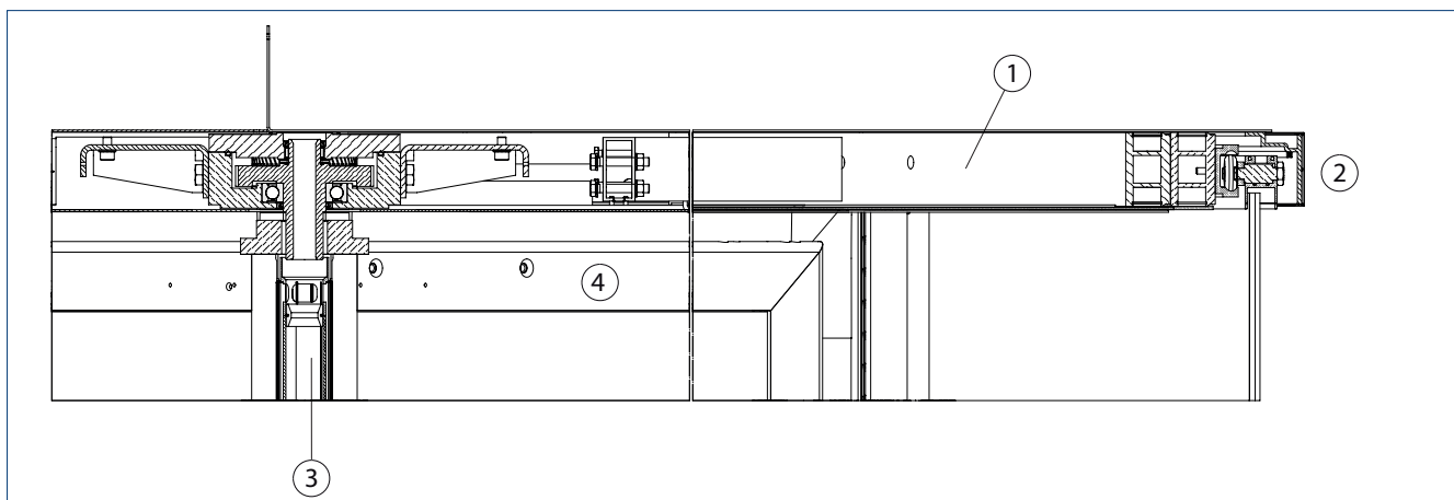
1 = Ceiling construction | 2 = Canopy profile with night-time closer on the outside | 3 = Swivelling axis | 4 = Side-hung leaf
