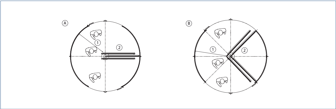
Revo.PRIME BO variants A = Three-leaf | B = Four-leaf | 1 = Escape route width | 2 = Leaf opened
